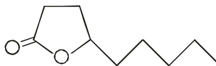
Dihydro-5-pentyl-Furanone
